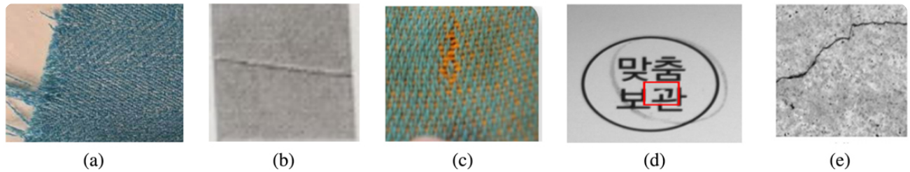
Figure from Nahar et al. (2026) showing defect examples: (a) fray on fabric (b) crease on steel (c) color imperfection on fabric, (d) silk screen printing and (e) crack on metal surface. CC BY 4.0 .
